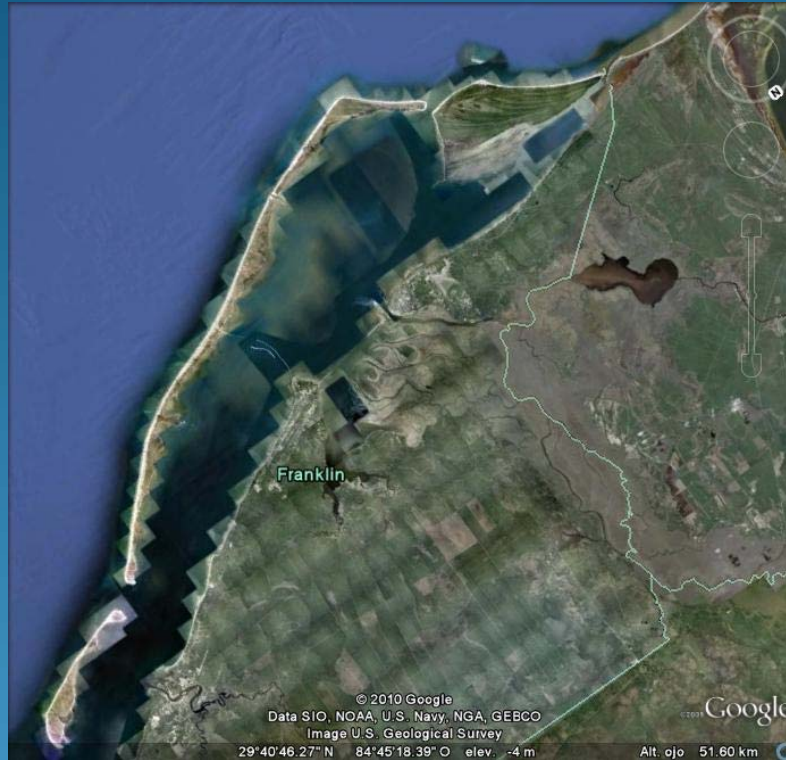
Barrier and lagoon, Jacksonville
