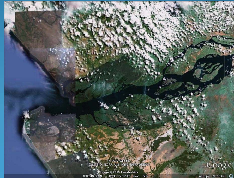
Cañón submarino, Congo
