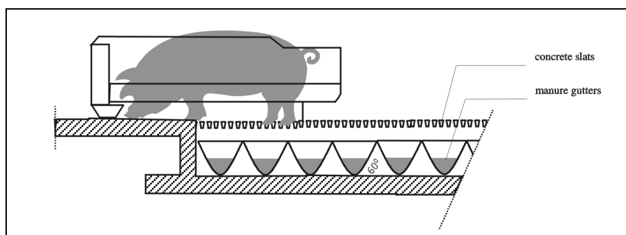
Figure 4.26: Partly-slatted floor with flushing gutter in individual housing situation [10, Netherlands, 1999]
