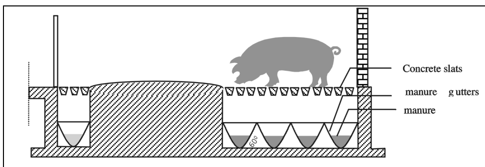
Figure 4.47: Convex floor with concrete (or triangular iron) slats in combination with a gutter system [10, Netherlands, 1999]
