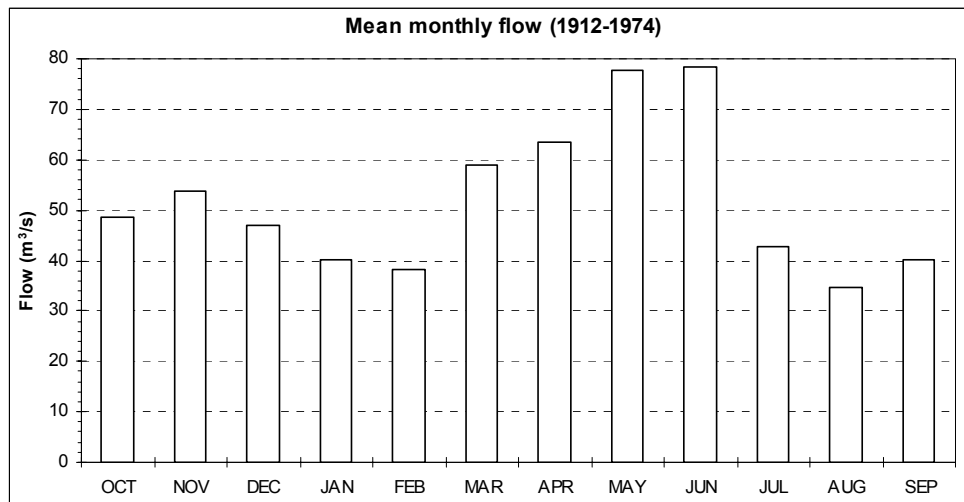
Figure 5-. Mean monthly flow in El Grado (Cinca River)
