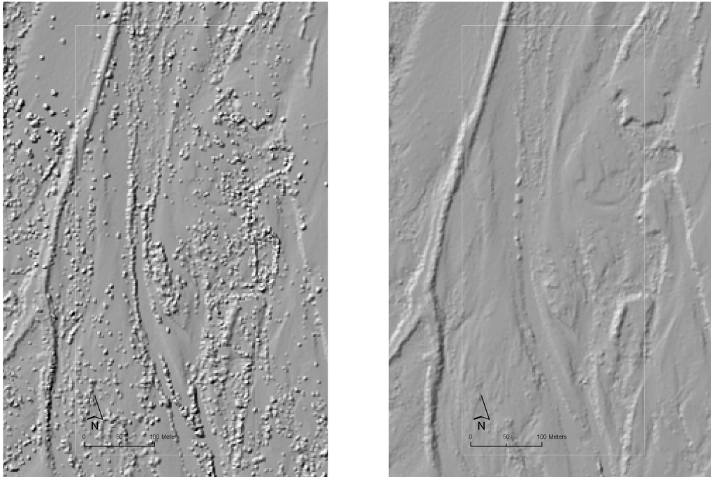
Figure 3-. Grids dsm (left) and dtm (right) for the selected reach (rectangle) in Cinca River
