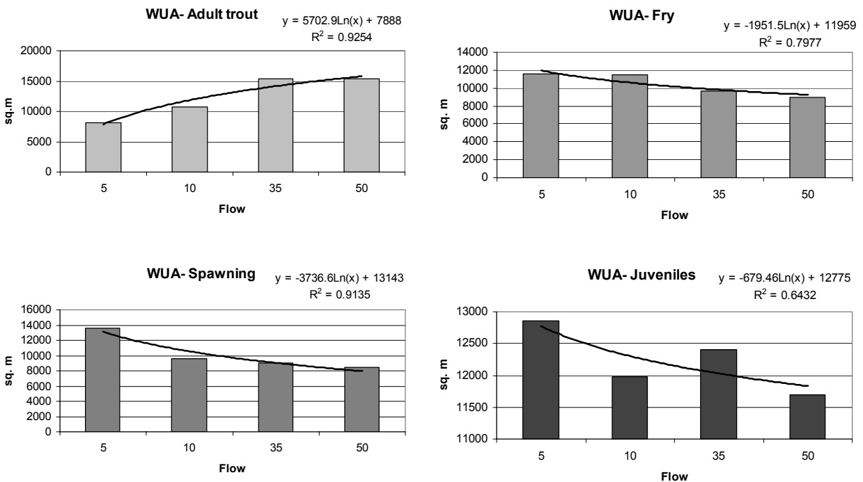
Figure 8-. Graphic quantification of brown trout habitat (Weighted usable area) for different simulated flows and regression expressions
