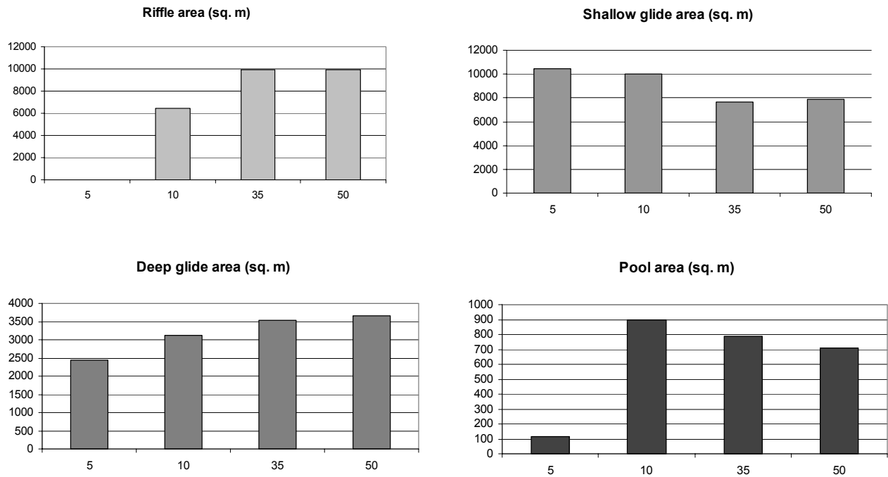
Figure 7-. Graphic quantification of mesohabitat units for different simulated flows
