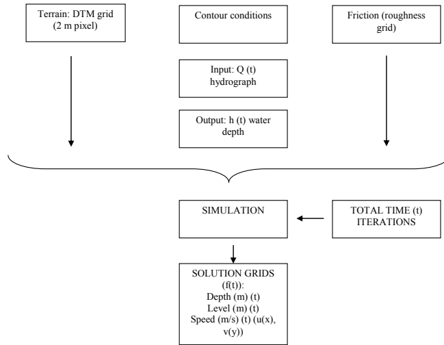
Figure 4-. Scheme for the hydraulic simulation with GUAD 2D
